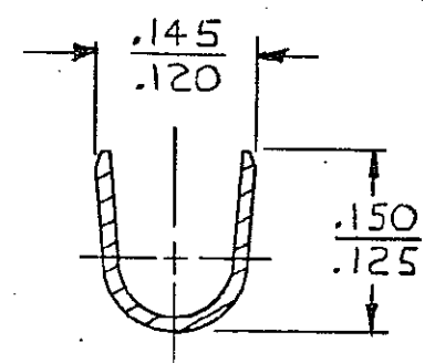
SECTION A-A SECTION B-B
